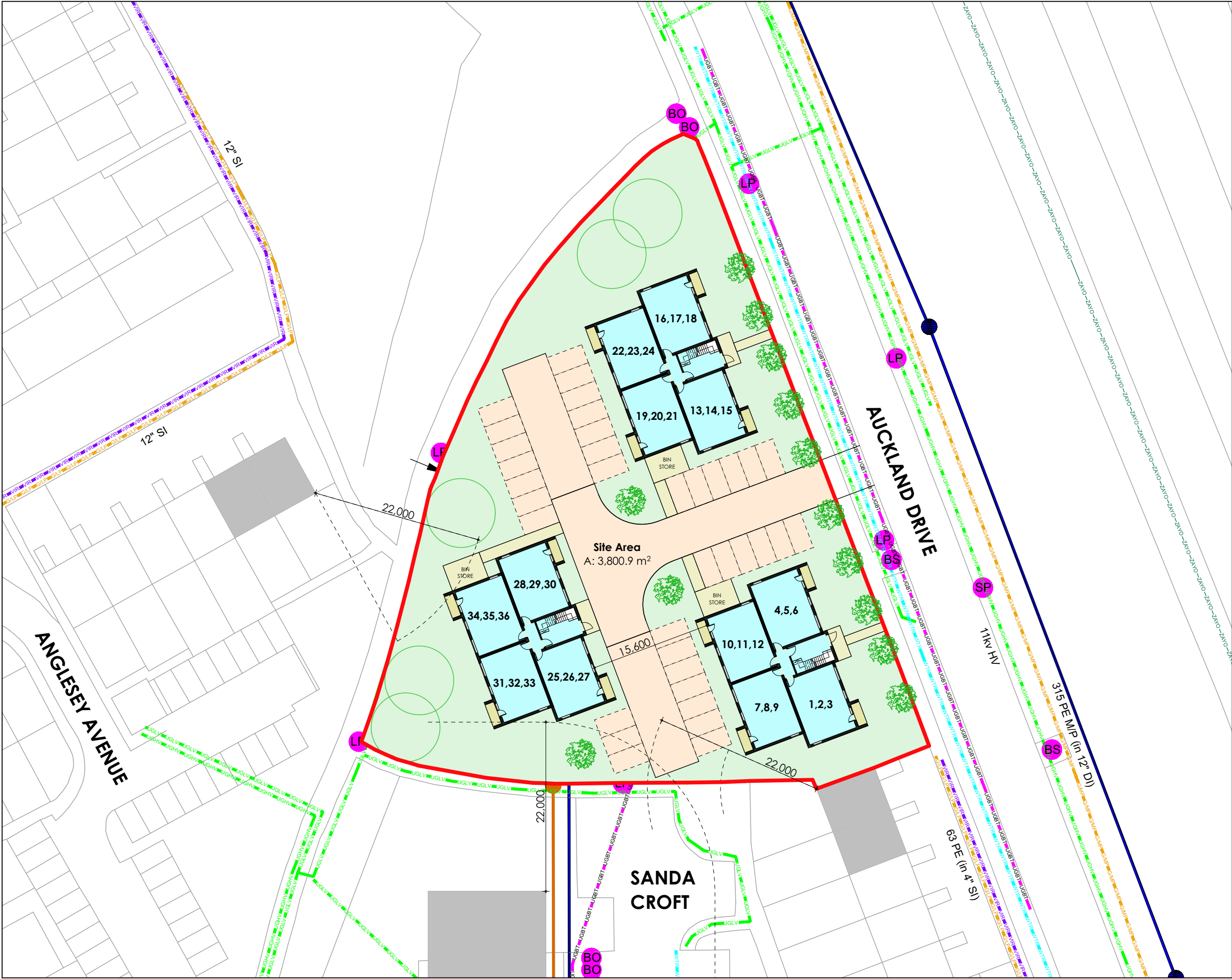
SITE PLAN
